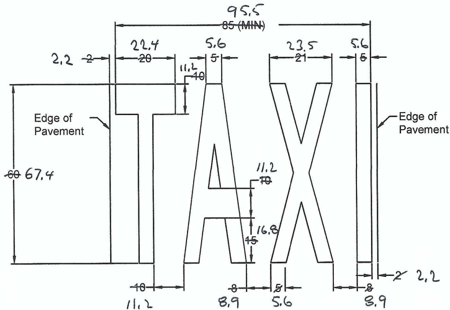
Figure 2. TAXI Marking Dimensions
